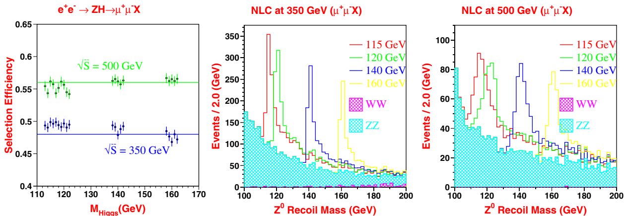
FIG. 1: Left – selection efficiency of e^+e^- \rightarrow Z^0H \rightarrow \mu^+\mu^-X plotted vs Higgs mass between 113 and 162 GeV. Green points are signal efficiencies at \sqrt{s} = 500 GeV and blue points are for \sqrt{s} = 350 GeV. Center – the recoil mass distributions of e^+e^- \rightarrow Z^0H \rightarrow \mu^+\mu^-X for Higgs boson masses at 115(red), 120(green), 140(blue) and 160(yellow) GeV, along with the background contributions from Z^0Z^0 (cyan) and W^+W^- (magenta) at \sqrt{s} = 350 GeV. Right – the corresponding recoil mass distributions at \sqrt{s} = 500 GeV.
