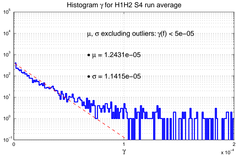
Figure 9: Same as above, but we remove the outlier jobs, the frequencies below 50 Hz, and the 60 Hz harmonics.
