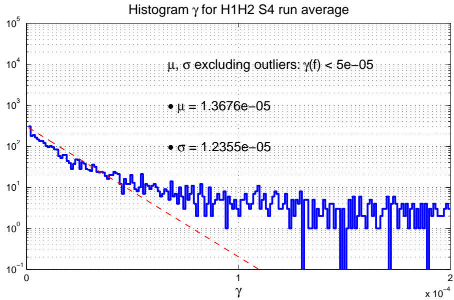
Figure 8: Top: Coherence vs frequency (including outliers). The black lines denote positions of pulsar injections. Bottom: Histogram of the coherence - note that it follows the expected exponential behavior at low \gamma values, but that it deviates from the exponential at large gamma values.
