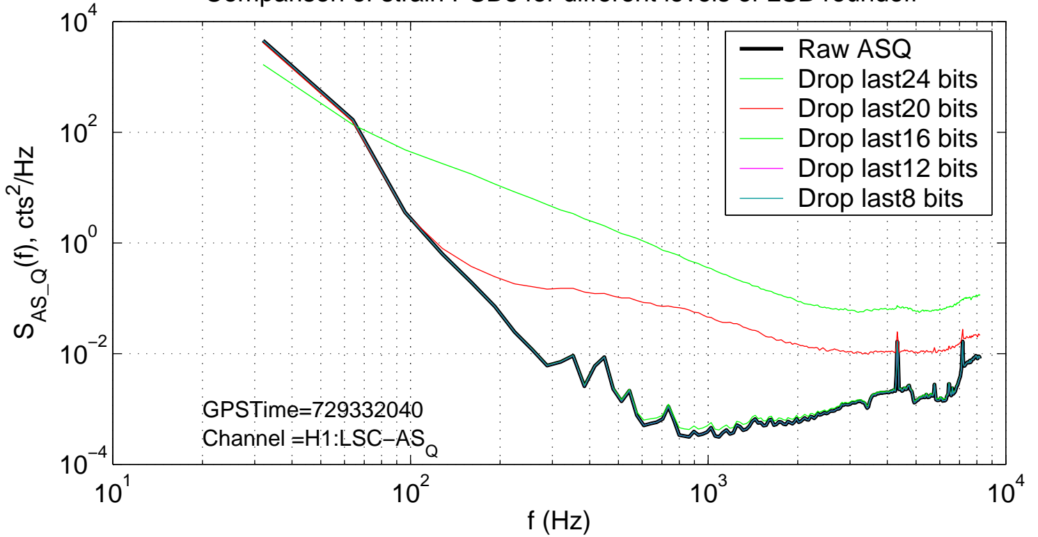
Comparison of strain PSDs for different levels of LSB roundoff
