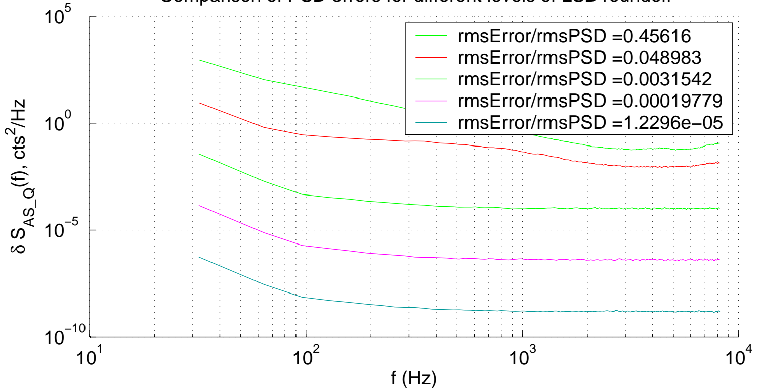
Comparison of PSD errors for different levels of LSB roundoff
