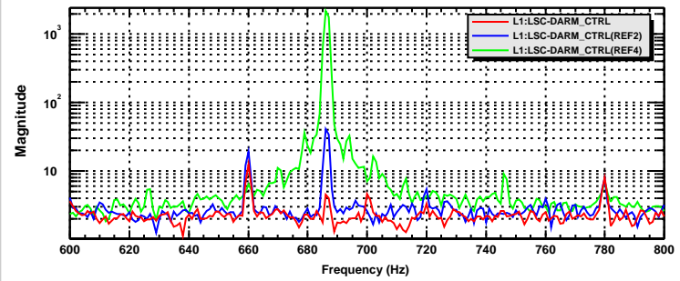
Power spectrum
