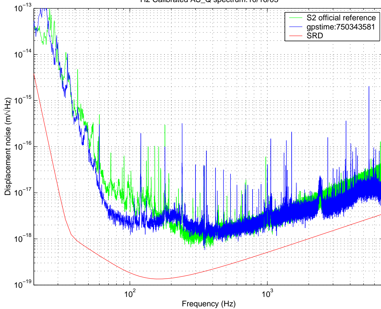
H2 Calibrated AS_Q spectrum:10/16/03
