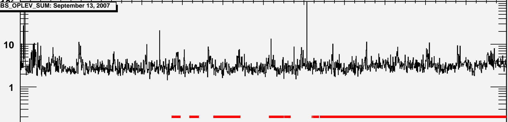
L1:SUS-BS_OPLEV_SUM: September 14, 2007
