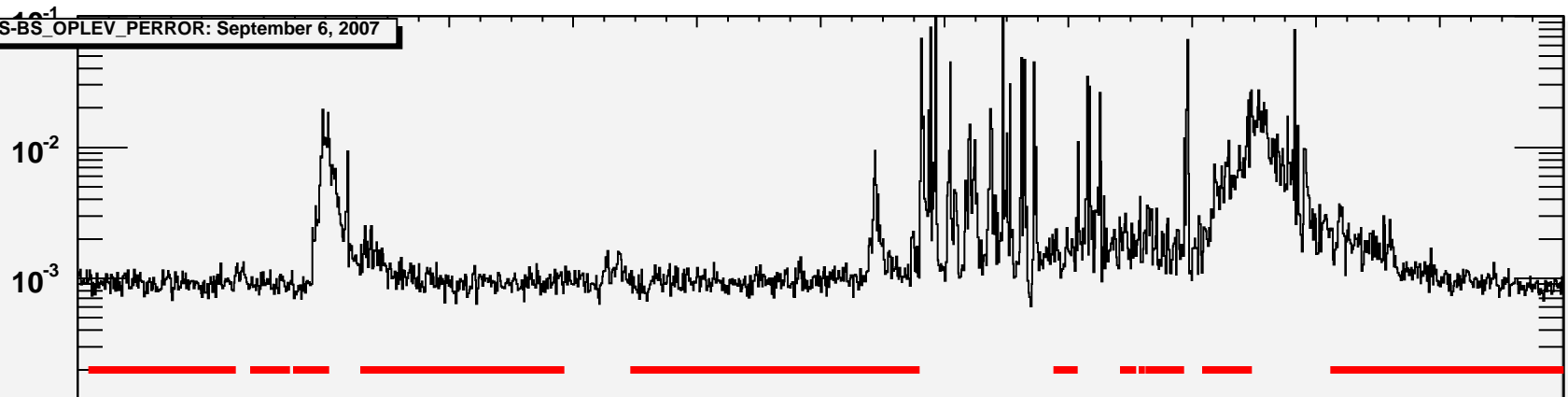
L1:SUS-BS_OPLEV_PERROR: September 7, 2007
