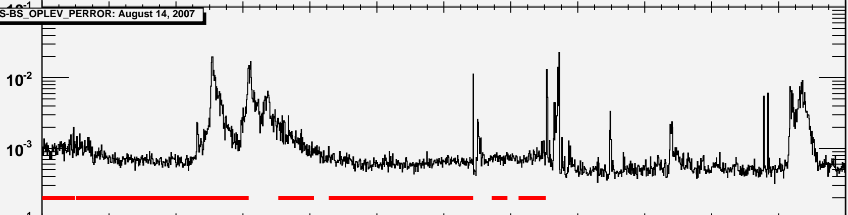
L1:SUS-BS_OPLEV_PERROR: August 15, 2007
