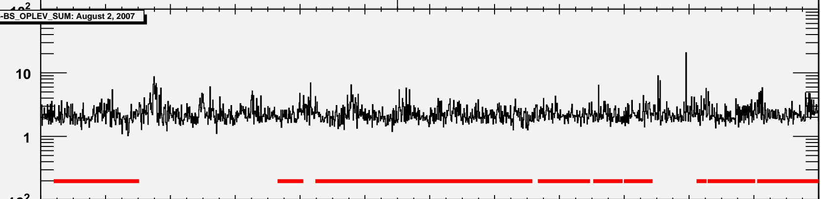
L1:SUS-BS_OPLEV_SUM: August 3, 2007
