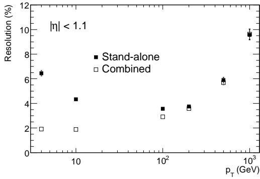
Figure 10.35: Expected stand-alone and combined fractional momentum resolution as a function of p_T for single muons with |\eta| < 1.1 .
