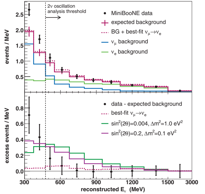
FIG. 2 (color). The top plot shows the number of candidate \nu_e events as a function of E_{\nu}^{\text{QE}} . The points represent the data with statistical error, while the histogram is the expected background with systematic errors from all sources. The vertical dashed line indicates the threshold used in the two-neutrino oscillation analysis. Also shown are the best-fit oscillation spectrum (dashed histogram) and the background contributions from \nu_{\mu} and \nu_e events. The bottom plot shows the number of events with the predicted background subtracted as a function of E_{\nu}^{\text{QE}} , where the points represent the data with total errors and the two histograms correspond to LSND solutions at high and low \Delta m^2 .
