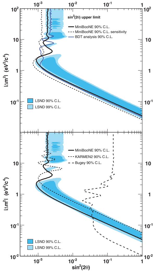
FIG. 3 (color). The top plot shows the MiniBooNE 90% C.L. limit (thick solid curve) and sensitivity (dashed curve) for events with 475 < E_{\nu}^{\text{QE}} < 3000 MeV within a two-neutrino oscillation model. Also shown is the limit from the boosted decision tree analysis (thin solid curve) for events with 300 < E_{\nu}^{\text{QE}} < 3000 MeV. The bottom plot shows the limits from the KARMEN [2] and Bugey [32] experiments. The MiniBooNE and Bugey curves are 1-sided upper limits on \sin^2 2\theta corresponding to \Delta\chi^2 = 1.64 , while the KARMEN curve is a “unified approach” 2D contour. The shaded areas show the 90% and 99% C.L. allowed regions from the LSND experiment.
