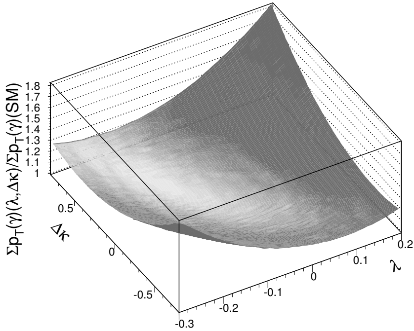
Figure 59: Dependence on the anomalous \Delta\kappa_\gamma and \lambda_\gamma parameters is illustrated by the ratio of production cross section to the Standard Model for W^\pm\gamma of with E_T(\gamma) > 50 GeV
