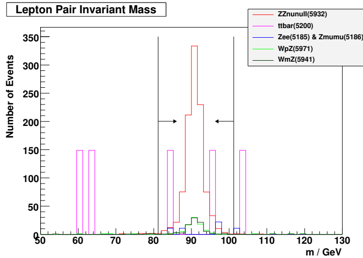
Figure 91: The lepton pair invariant mass distribution after all cuts except for the mass window restriction. The histograms have been scaled to represent the number of events expected in 100 \text{ fb}^{-1} of data.
