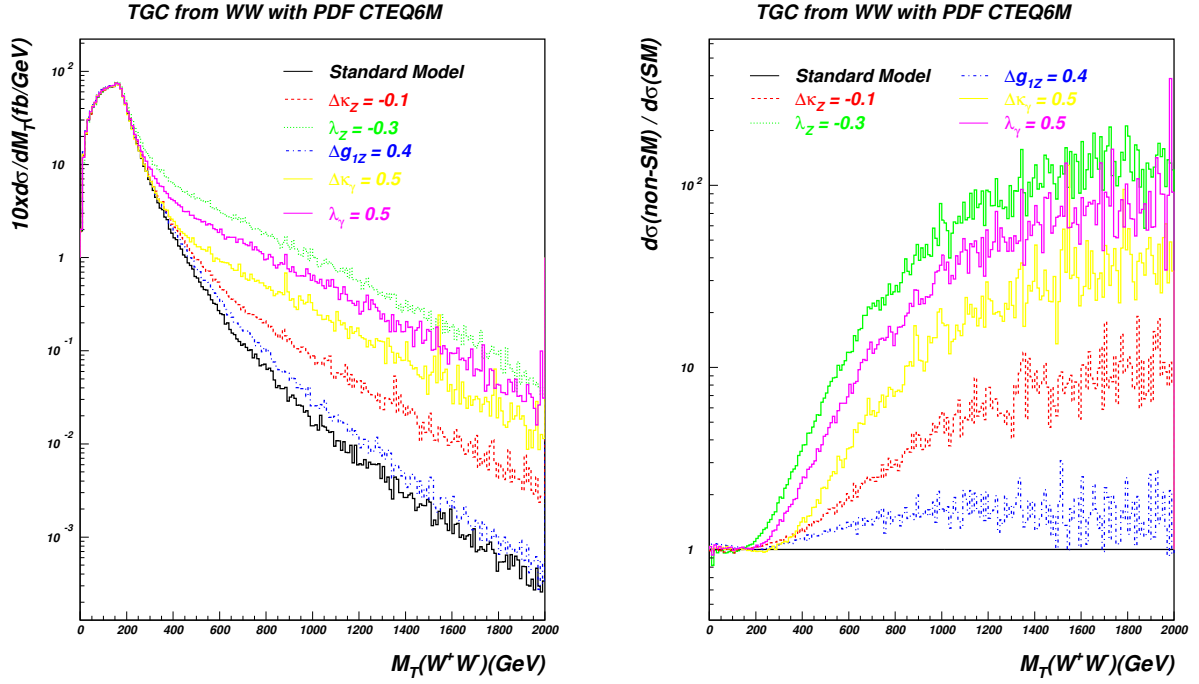
Figure 21: Left: WW transverse mass, M_T , distributions. Events are generated with the SM coupling (black) and anomalous couplings (color); Right: the corresponding differential cross section ratio, d\sigma(\text{non-SM})/d\sigma(\text{SM}) .
