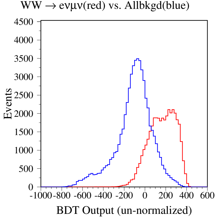
Figure 15: Distributions of the BDT -output spectra. Red histogram is for WW signal events, and the blue, is for all the background.
