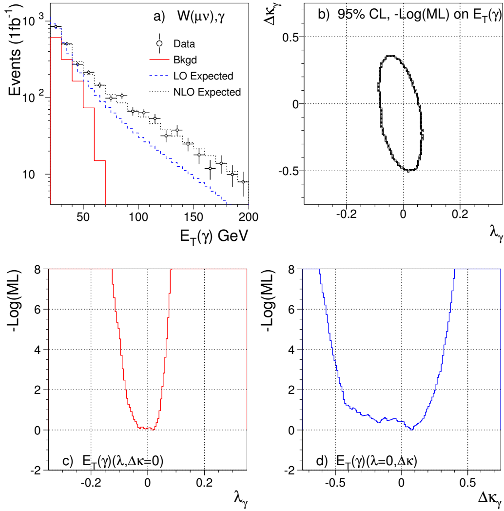
Figure 60: The Log likelihood was calculated for the E_T(\gamma) distribution of NLO expectation of 1\text{fb}^{-1} of data in a). The 95 % confidence contour is plotted in b), and the log likelihood functions of \lambda_\gamma and \Delta\kappa_\gamma are plotted in c) and d), respectively.
