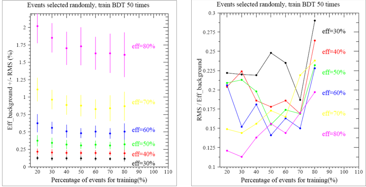
Figure 40: Left figure: Background acceptance as a function of percentage of events used for BDT training for given signal efficiencies. Each point presented in the plot is averaged from 50 times randomly selected events samples for test. The error bar is the standard deviation (RMS) of the mean value. Right: Relative errors as a function of the percentage of the training samples.
