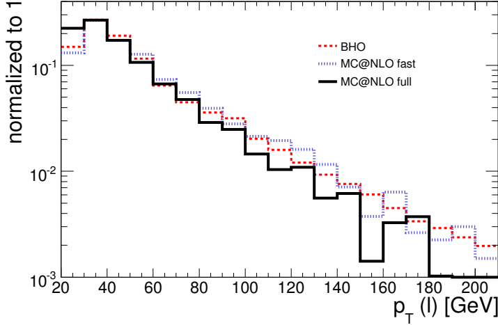
Figure 99: BHO and MC@NLO predictions for lepton p_T distribution after fast simulation of ATLAS detector and "B" selection (section 4.4.1).
