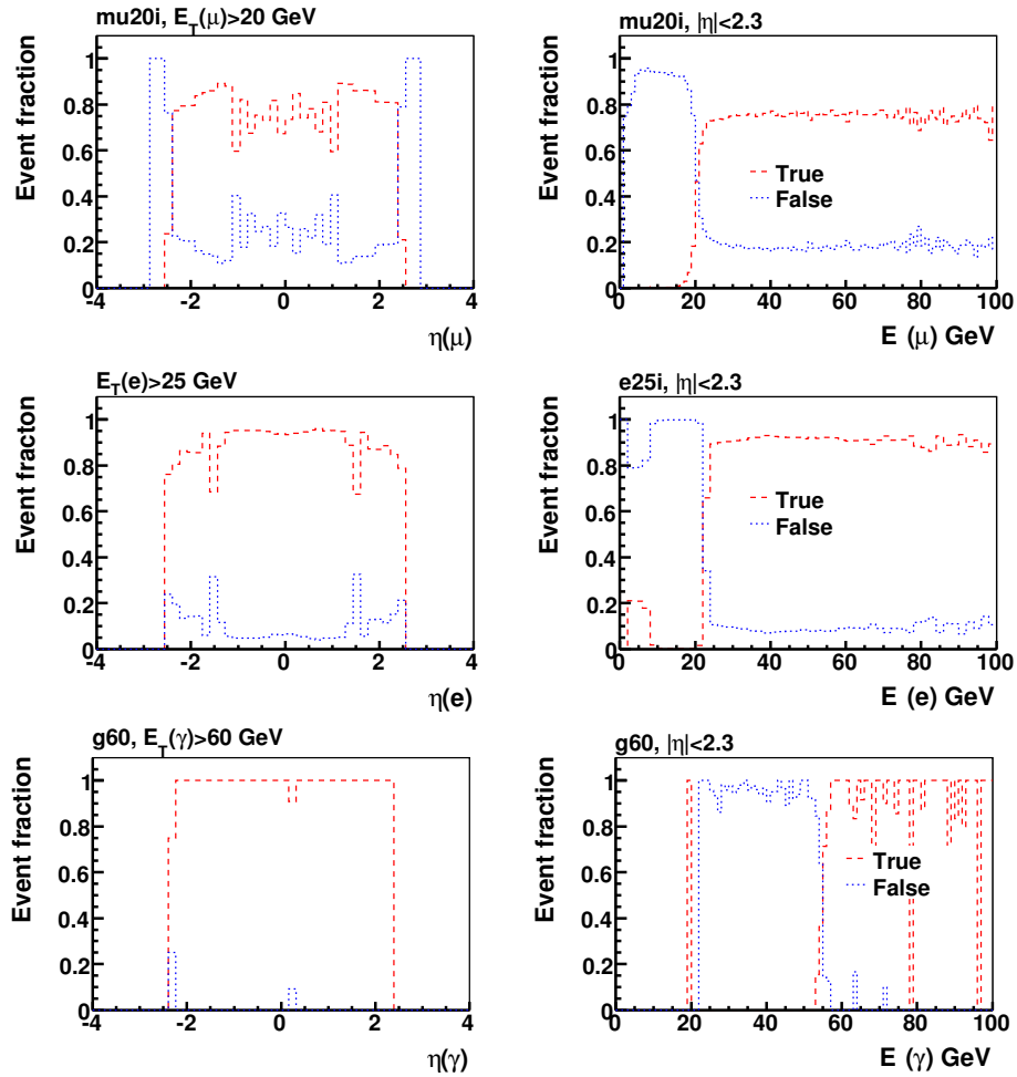
Figure 50: Trigger efficiencies of mu20i, e25i and g60 estimated with W^\pm decay leptons and ISR photons. The reference are the muons, electrons, and photons of muon_boy and lsEM 0x7FF reconstruction that match with MCtruth.
