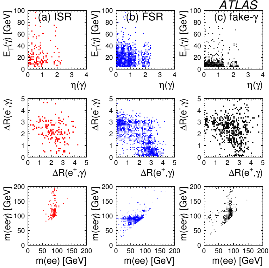
Figure 64: Distributions of Z(ee)\gamma event variables with ISR, FSR and fake photons.
