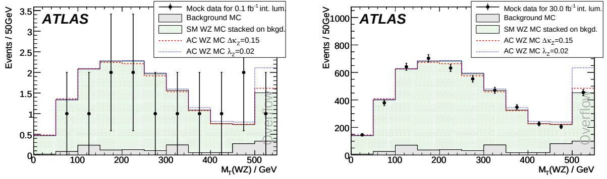
Figure 44: The expected signal+background of the SM, superimposed with the MC experiment “observations” (points with error bars showing statistical uncertainty), and the non-SM (anomalous couplings) predicted signal+background histograms (red and blue dashed lines). the left plot is for 0.1\text{fb}^{-1} and the right plot is for 30\text{fb}^{-1} .
