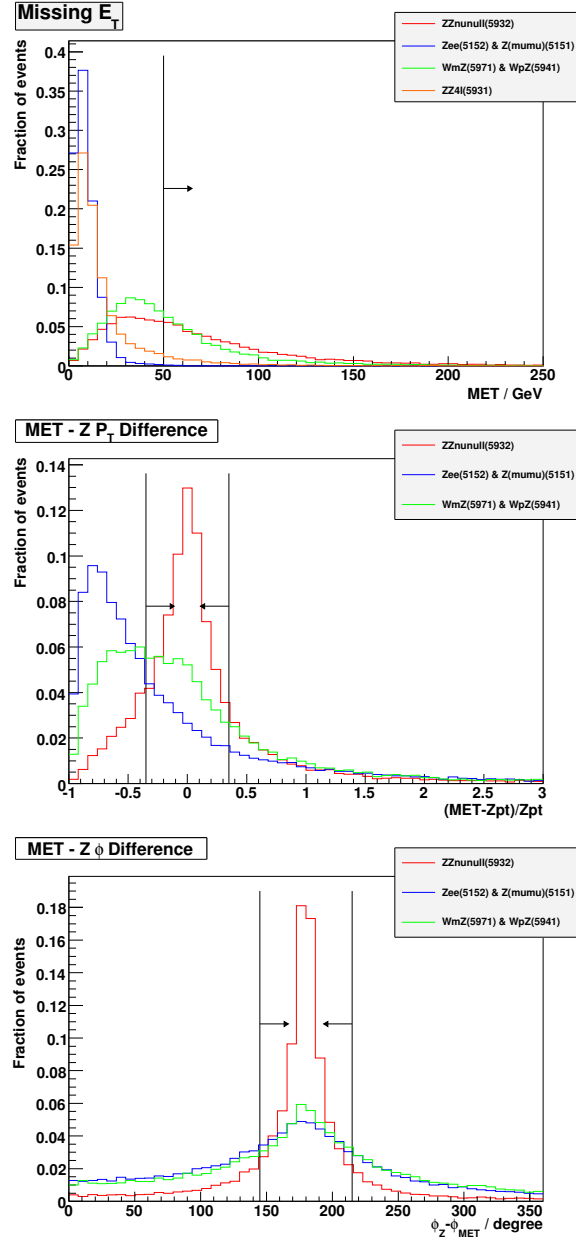
Figure 88: The \cancel{E}_T and \cancel{E}_T - p_T(Z) magnitude and angle matching distributions before cuts for the signal (red), ZZ \rightarrow 4\ell (orange), Z \rightarrow \ell^+\ell^- (blue) and W^\pm Z (green) using version 12 data. The plots are normalised to unit area for comparison of distribution shapes.
