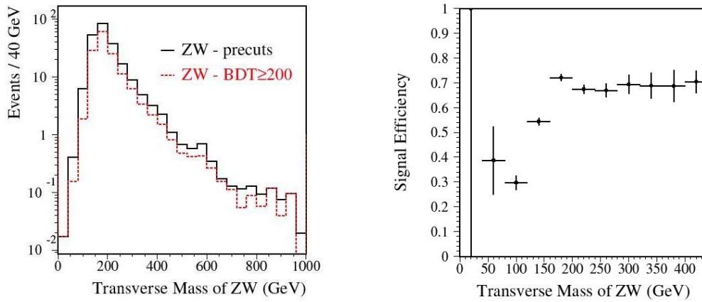
Figure 37: Distribution of transverse mass of W^\pm Z before and after the BDT selection (left); Selection efficiency ( BDT > 200 ) as a function of the transverse mass of W^\pm Z (right).
