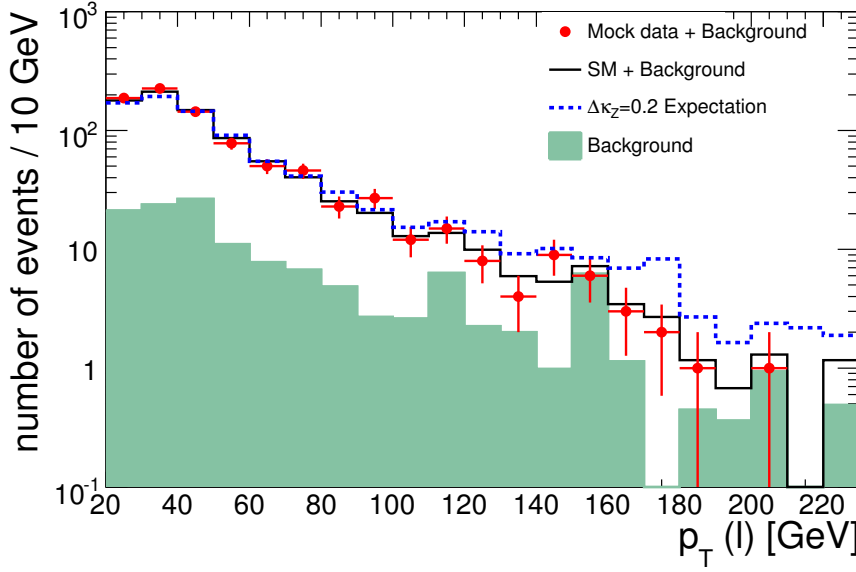
Figure 100: The transverse momentum distribution of leptons after applying the kinematic cuts. The points with error bars represent "mock" data with integrated luminosity of 10 \text{ fb}^{-1} . The lines are SM MC distribution and \Delta\kappa_Z = 0.2 theoretical expectation. The contribution of all backgrounds to reference distributions is shown as a shaded histogram.
