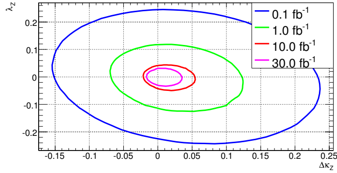
Figure 25: Two-dimensional anomalous coupling parameters fitting for 0.1 - 30 \text{fb}^{-1} MC data based on the HISZ assumption to relate the coupling parameters.
