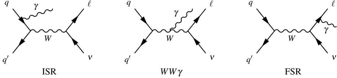
Figure 48: Feynman diagrams for W^\pm\gamma production. The W production with the ISR (initial state radiation) and the W radiating a photon with the WW\gamma vertex (left and middle diagrams) are considered as our signal. The right diagram is the W production with a photon radiating from the final state lepton (FSR), which is considered as the W^\pm\gamma background.
