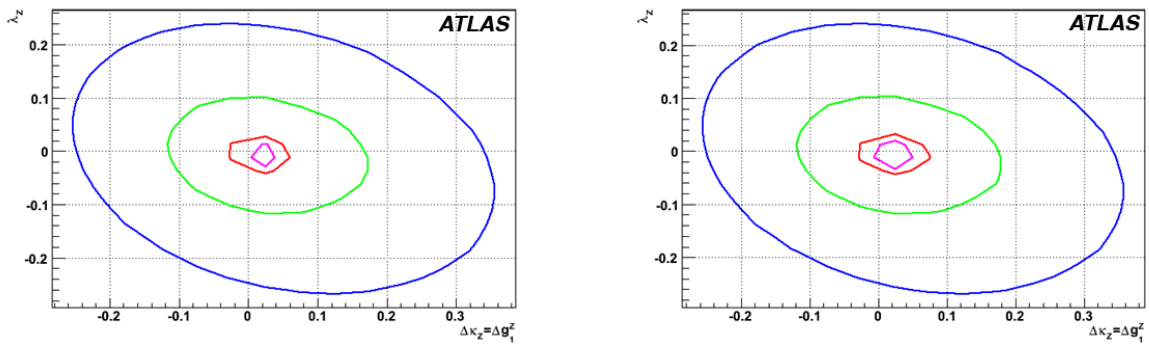
Figure 47: The left plot: 95% C.L. WWZ TGC limit contour without including the systematic errors in parameter space of \lambda_Z vs. \Delta\kappa_Z = \Delta g_1^Z ; The right plot: the 95% C.L. WWZ TGC limit contour with the systematic errors ( \sigma_S = 9.2\% , \sigma_B = 18.3\% ) in parameter space of \lambda_Z vs. \Delta\kappa_Z = \Delta g_1^Z . The AC limit contours from outer to inner corresponding integrated luminosities of 0.1, 1.0, 10.0 and 30.0 \text{fb}^{-1} , respectively. We should notice that the systematic errors become significant when integrated luminosity reaching 30 \text{fb}^{-1} .
