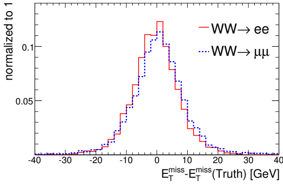
Figure 7: \cancel{E}_T resolution for WW \rightarrow ee and WW \rightarrow \mu\mu .
