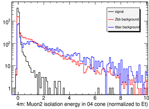
(c) Isolation variable I (see text) for the 2nd highest p_T muon
