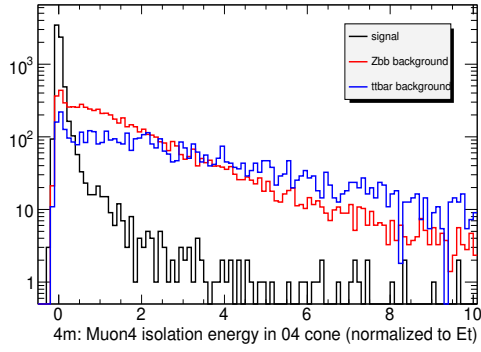
(a) Isolation variable I (see text) for the softest muon
