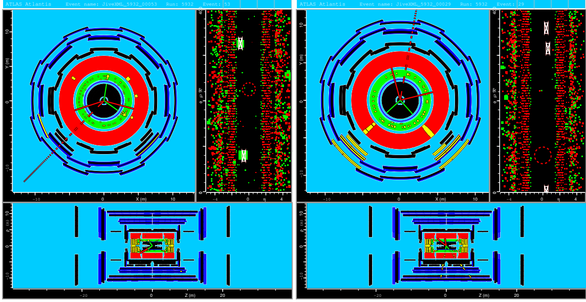
Figure 81: Monte Carlo ZZ \rightarrow \ell\ell\nu\bar{\nu} events shown by the ATLAS event display, Atlantis. The left-hand diagram is an example of an electron event, while the right-hand diagram shows a corresponding muon example. Both diagrams show the x - y plane (top-left panel), the \eta - \phi plane (top-right panel) and the x - z plane (lower panel). The inner detector is shown by the black central region, with the EM-calorimeter in green, the hadron calorimeter in red and the muon system in blue. The green lines depict reconstructed tracks, while red solid lines represent the true neutrino tracks. The red dashed line shows the direction of the missing transverse energy. Calorimeter deposits and muon chambers containing hits are highlighted in yellow.
