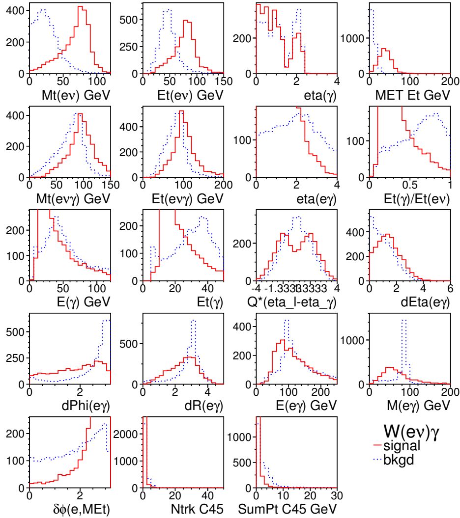
Figure 52: Distributions of event variables used in Boosted decision tree for W^\pm(e^\pm\nu)\gamma with signal of ISR photons and background of inclusive Z(ee) contamination.
