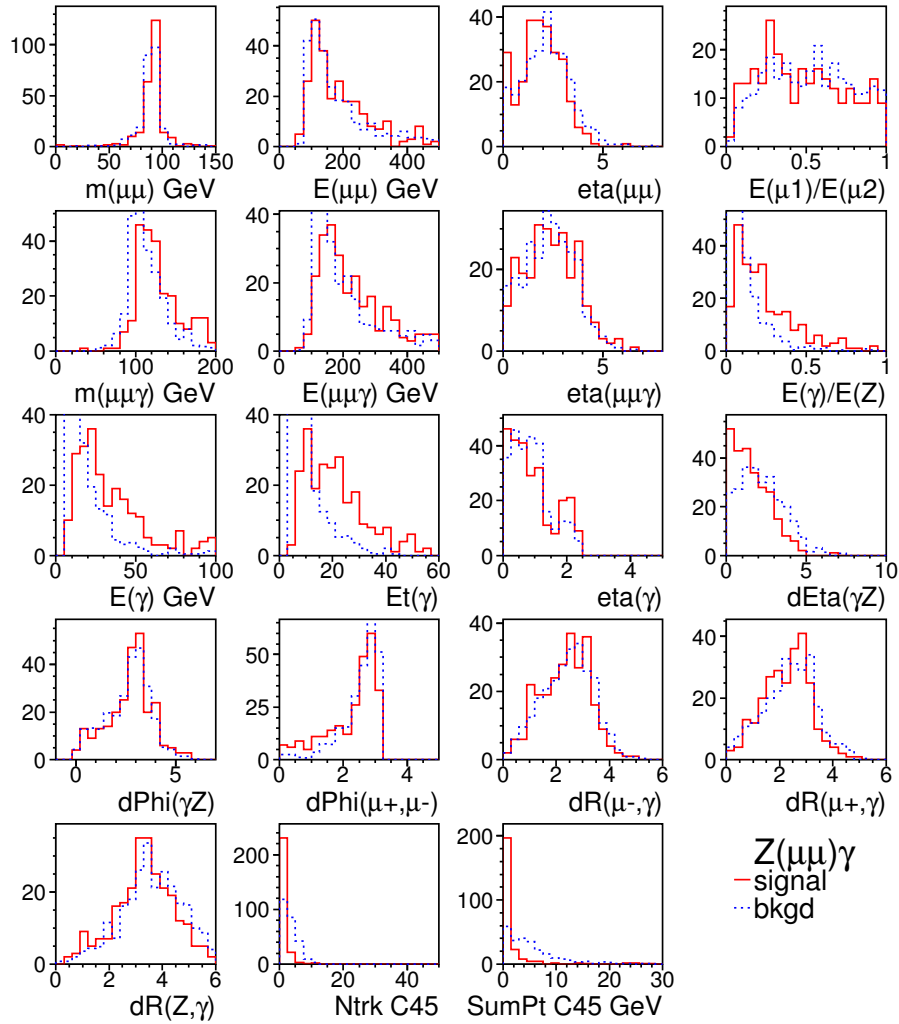
Figure 66: Distributions of variables used in Boosted decision tree for selection of Z(\mu^+\mu^-)\gamma events with signal of ISR photons and background of fake photons.
