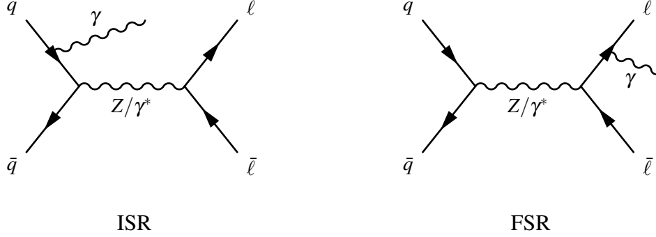
Figure 61: Born diagrams of the Z\gamma production in hadron collider.
