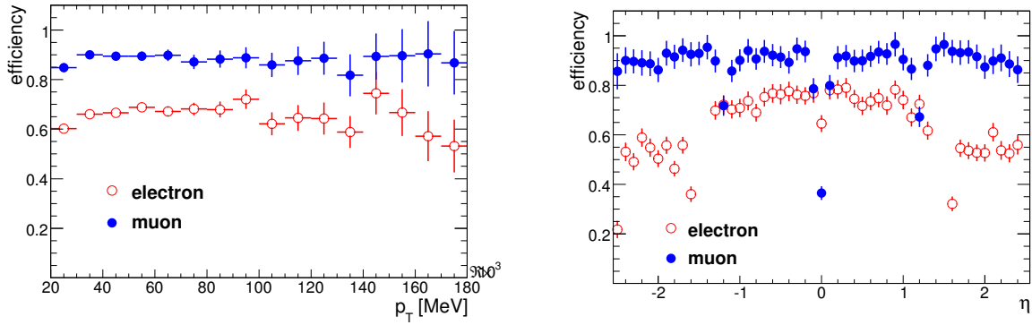
Figure 4: Electron and muon reconstruction efficiencies as a function of p_T (left) and \eta (right).
