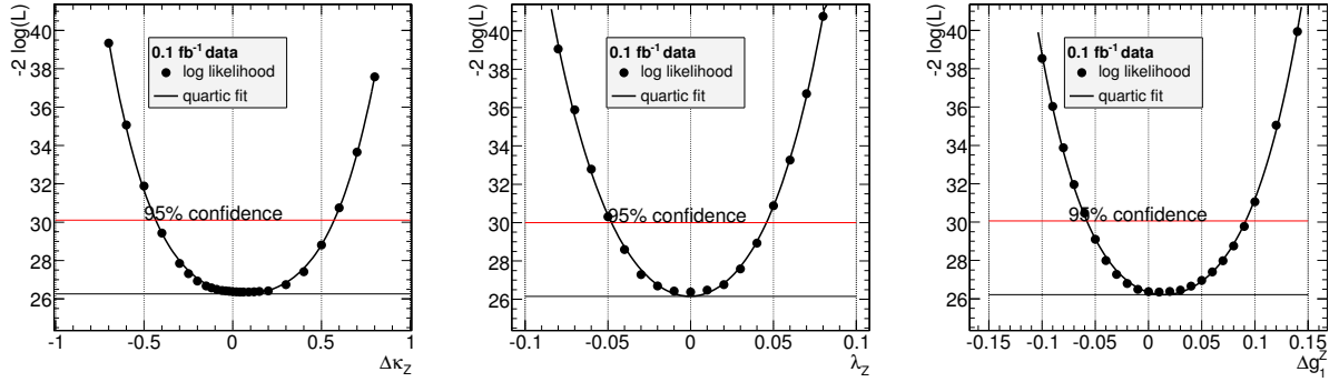
Figure 45: One-dimensional anomalous coupling likelihood fits for \Lambda = 3 TeV using M_T(W^\pm Z) spectra from 0.1\text{fb}^{-1} data. When varying one anomalous coupling parameter for fitting, the other parameters are fixed to SM values.
