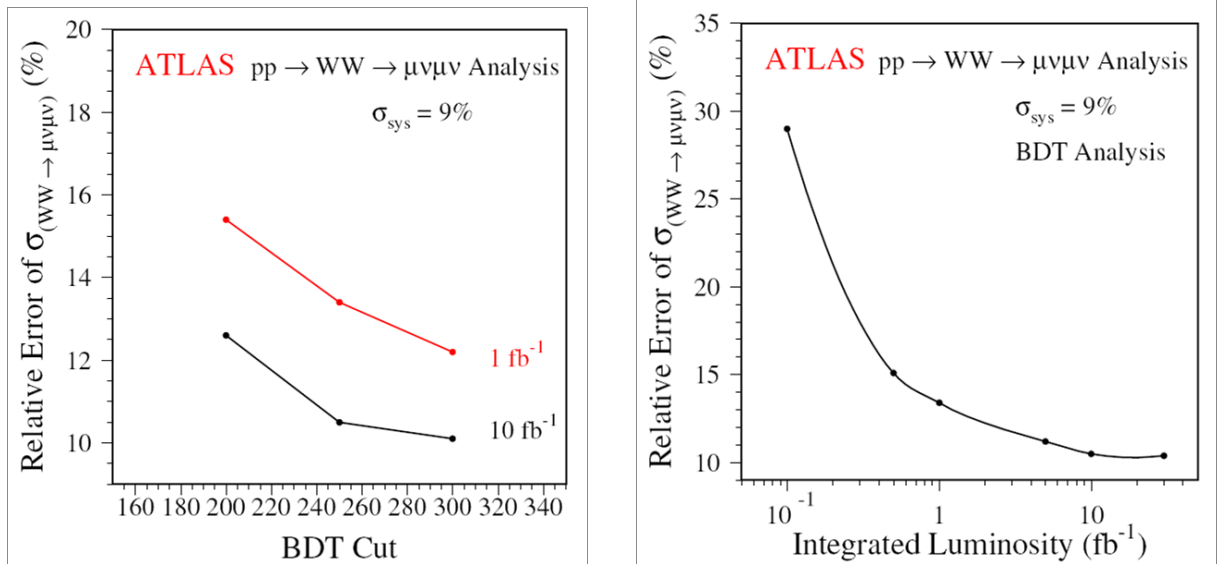
Figure 20: Left plot: the relative errors for cross section measurement as a function of the BDT cut. The optimal BDT spectrum cut should be around 240. Right plot: the relative errors as a function of integrated luminosity (with the BDT spectrum cut at 240). From this plot, we see that systematic error starts to dominate after 10 \text{ fb}^{-1} integrated luminosity.
