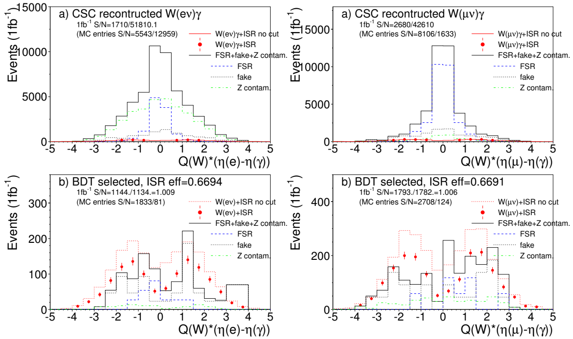
Figure 56: Distributions of Q_W \cdot (\eta(l) - \eta(\gamma)) for reconstructed W^\pm\gamma candidates (upper row) and after decision tree cuts (lower row), for W^\pm decays in electron (left) and muon (right) channels. The distributions are normalized (by about a factor two to ISR and a factor 14 to background) to the 1\text{fb}^{-1} expectation.
