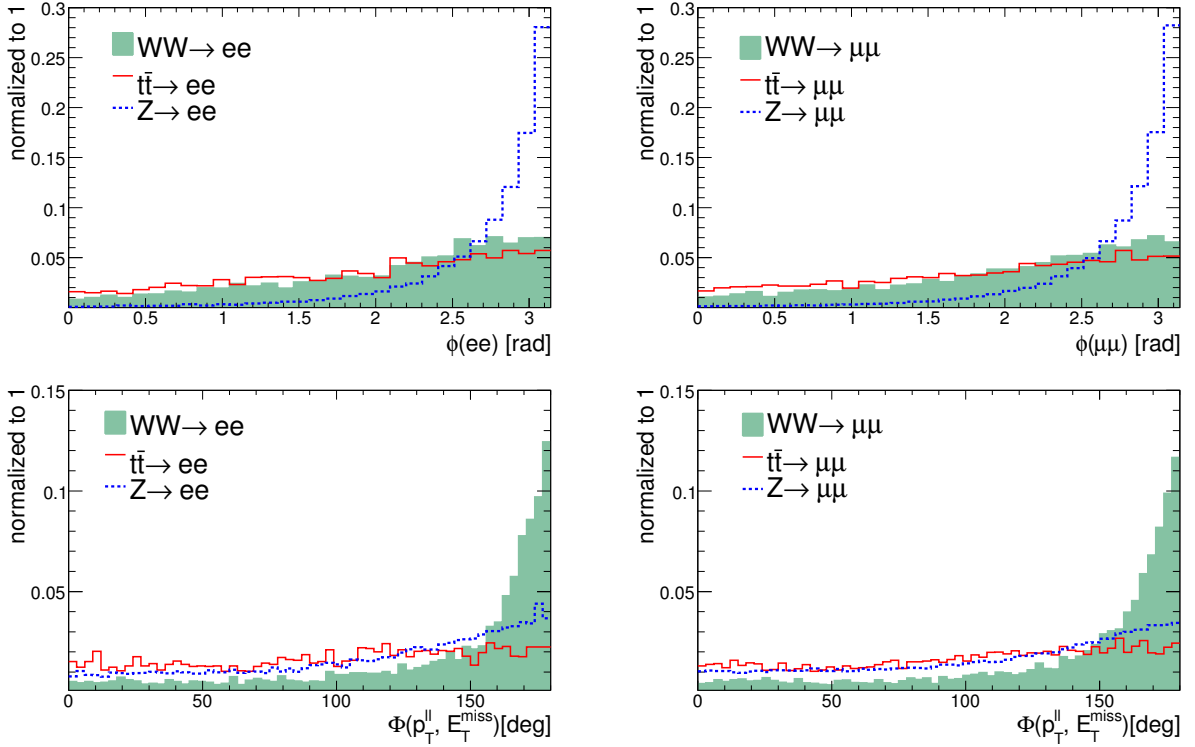
Figure 9: \phi(\ell^+\ell^-) and \Phi(p_T(\ell^+\ell^-), \cancel{p}_T) distributions for W^+W^- , t\bar{t} and Z/\gamma .
