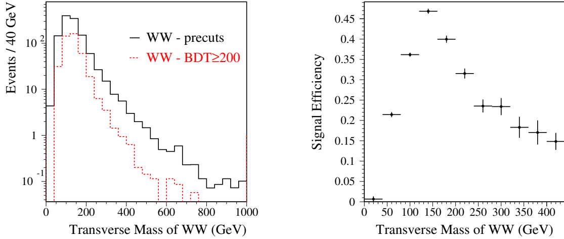
Figure 16: The left plot: the distributions of the transverse mass of the W-pair ( M_T(WW) ) before and after the BDT-output cut ( > 200 ); The right plot: the BDT selection efficiency as a function of the M_T(WW) . The last bin is the sum of all the overflow bin.
