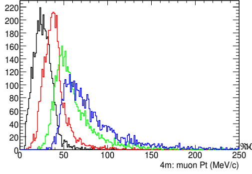
(a) Ordered p_T distributions of the 4 muons in 4\mu events.
