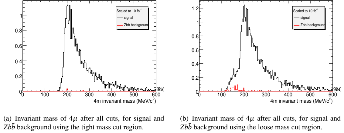
Figure 78: Invariant mass of 4\mu after all cuts, for signal and Zb\bar{b} background.
