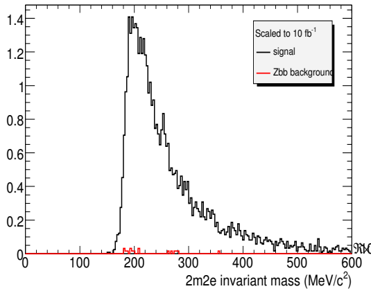
(a) Invariant mass of 2m2e after all cuts, for signal and Zb\bar{b} background using the tight mass cut region.
