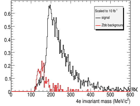
(b) Invariant mass of 4e after all cuts, for signal and Zb\bar{b} background using the loose mass cut region.
