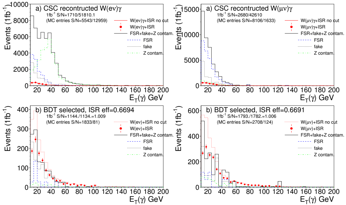
Figure 55: E_T(\gamma) distributions of reconstructed W^\pm\gamma events (upper row) and after decision tree cuts (lower row), for W^\pm decays into electron (left) and muon pairs (right). The distributions are normalized (by about a factor two to ISR and a factor 14 to background) to the 1\text{fb}^{-1} expectation.
