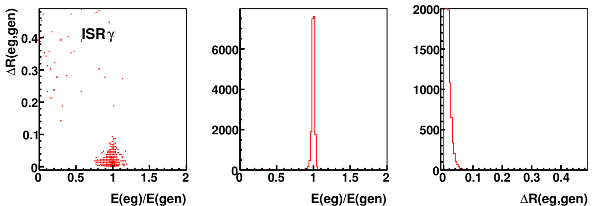
Figure 62: Plotted are the deviation in reconstructed energy and direction to the MCtruth parameters for ISR photons of E_T(\gamma) > 25 GeV
