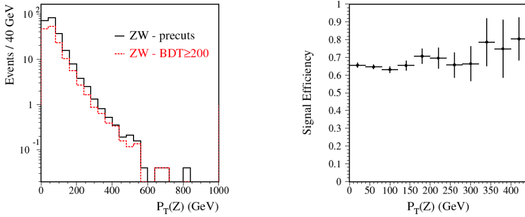
Figure 38: Transverse momentum distribution of the Z from W^\pm Z before and after the BDT cut (left); BDT selection efficiency as a function of transverse momentum of the Z (right).
