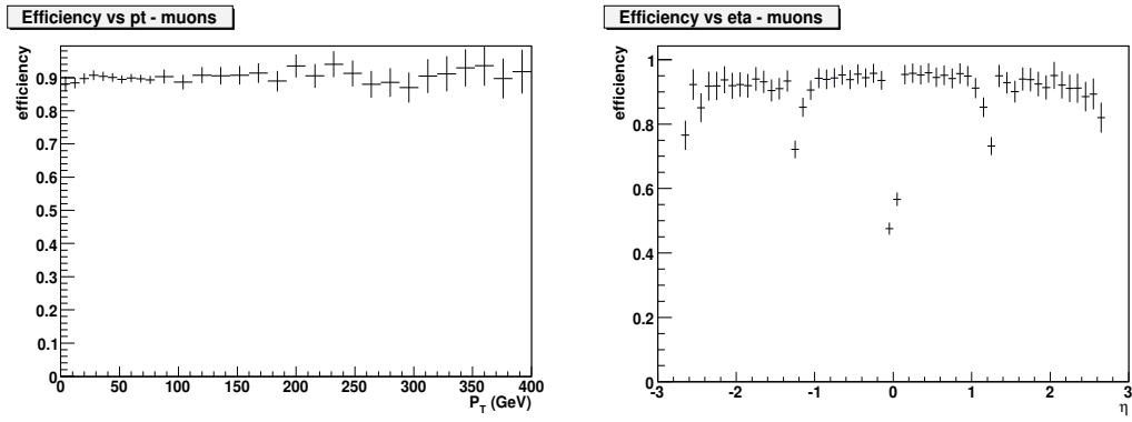
(a) p_T dependence of the muon reconstruction efficiency in ZZ events (b) \eta dependence of the muon reconstruction efficiency in ZZ events
