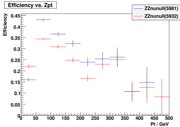
Figure 92: Signal selection efficiency against p_T(Z) for 11.0.4 and 12.0.6 Monte Carlo. The efficiency is defined as the number of reconstructed events passing selection cuts over the number of true events with p_T(l) > 20 \text{ GeV} , |\eta_l| < 2.5 and \cancel{E}_T > 50 \text{ GeV} .
