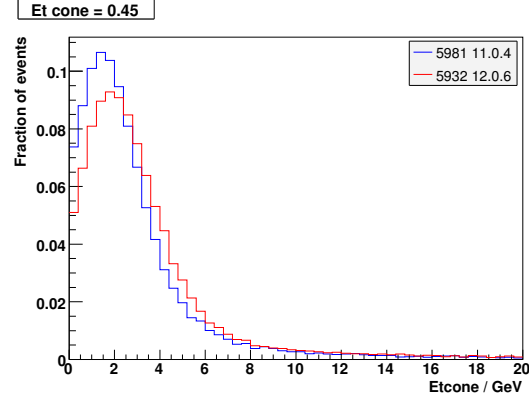
Figure 82: The distribution of transverse energy in a \Delta R = 0.45 cone around the electron track for electrons present in the signal ZZ \rightarrow \ell\ell\nu\bar{\nu} events. Version 11 data are shown in blue while version 12 data are in red.
