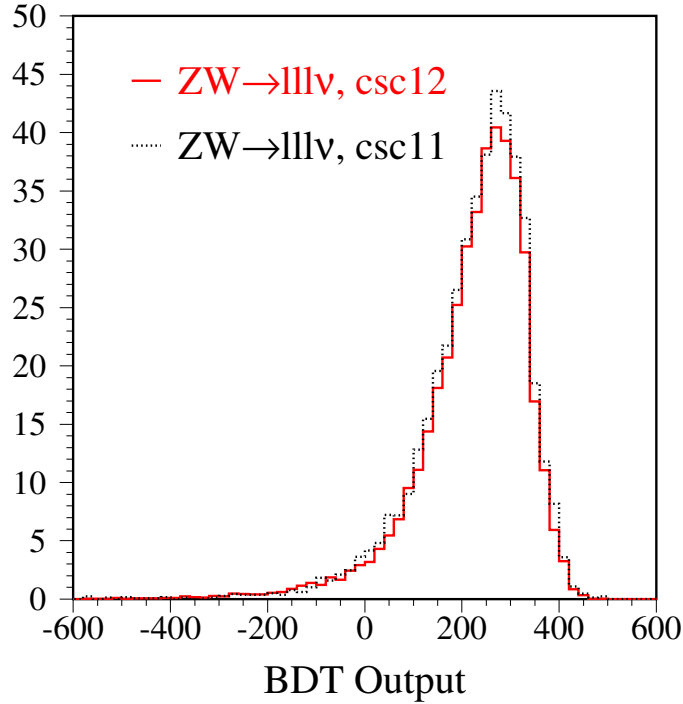
Figure 39: The BDT output spectra comparison: BDT training used CSC11 MC sample, and BDT test used both CSC11 and CSC12 samples. The output spectrum shows the stability of the BDT analysis technique.
