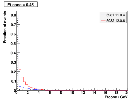
Figure 85: The distribution of transverse energy in a \Delta R = 0.45 cone around the muon track for version 11 (blue) and 12 (red) ZZ \rightarrow \ell\ell\nu\bar{\nu} signal datasets.
