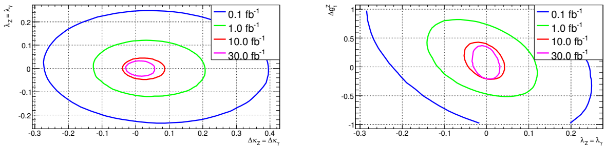
Figure 26: Two-dimensional anomalous coupling parameters fitting for 0.1 - 30 \text{fb}^{-1} MC data. For these fit, we have assumed Z = \gamma in parameter space: \Delta\kappa_Z = \Delta\kappa_\gamma , \lambda_Z = \lambda_\gamma .
