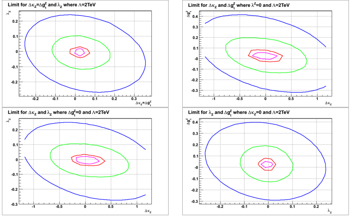
Figure 46: Two-dimensional 95% C.L. contour of the WWZ AC limits based on p_T(Z) fit for \Lambda = 2 TeV. The left-top plot shows the contour in \lambda_Z and \Delta\kappa_Z = \Delta g_1^Z space; the right-top plot shows the contour in \Delta\kappa_Z and \Delta g_1^Z space with (\lambda_Z = 0) ; the left-bottom plot shows the contour in \lambda_Z and \Delta\kappa_Z space with (\Delta g_1^Z = 0) ; the right-bottom plot shows the contour in \Delta g_1^Z and \lambda_Z space with (\Delta\kappa_Z = 0) . The AC limit contours from outer to inner corresponding integrated luminosities of 0.1, 1.0, 10.0 and 30.0 \text{fb}^{-1} , respectively.
