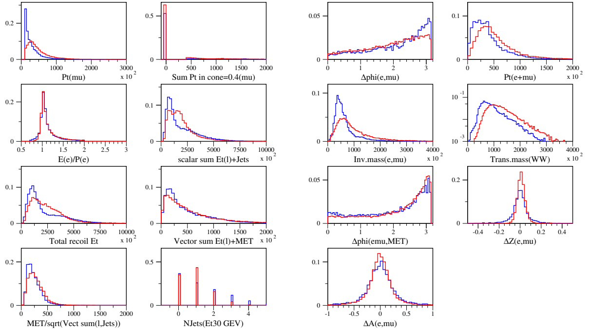
Figure 14: Distributions of the BDT training input variables for pre-selected W^\pm W^\mp \rightarrow e^\pm \nu \mu^\mp \nu candidates rejected because \text{BDT} < 200 . The histograms are normalized to unit area, red for the W^+W^- signal and blue for the total background.
