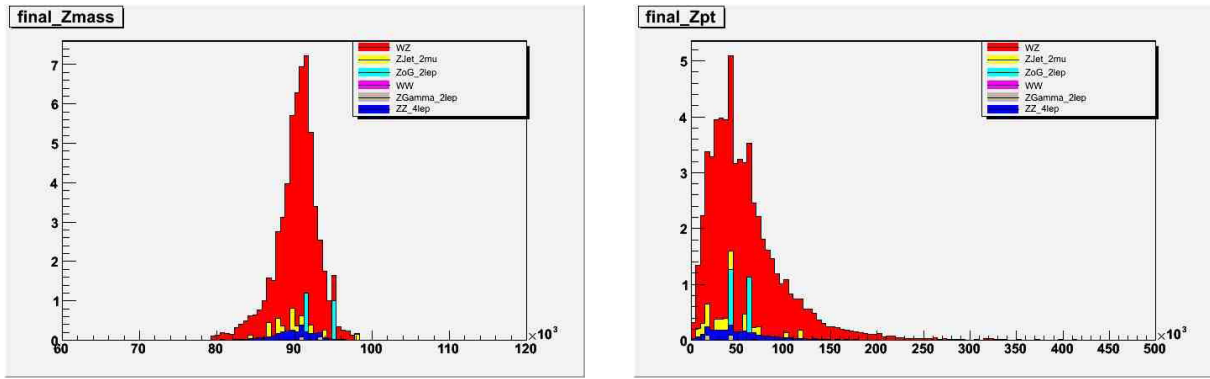
Figure 34: (a) left: Final selected dilepton invariant mass distributions. (b) right: p_T(Z) distributions with final selection. Number of events are normalized to 1\text{fb}^{-1} .
