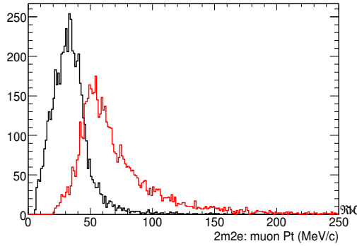
(c) Ordered p_T distributions of the 2 muons in 2\mu 2e events.
