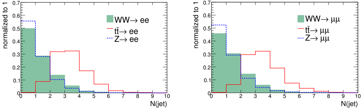
Figure 5: Jet multiplicity distribution in W^+W^- , t\bar{t} and Z/\gamma leptonic decay processes. Jets are reconstructed with an 0.7 cone, |\eta| < 3 , and E_T > 20 GeV.
