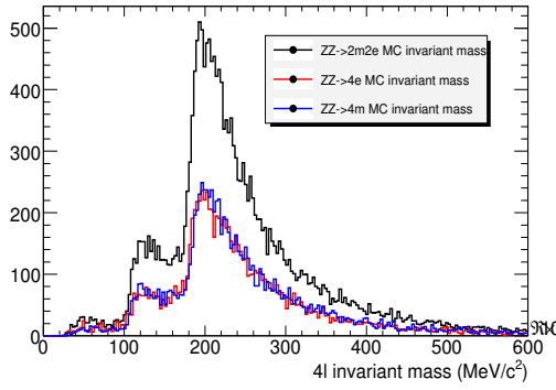
(a) The invariant mass distribution for ZZ \rightarrow 4\ell PYTHIA events for the three event categories : 4\mu , 4e and 2\mu 2e .
