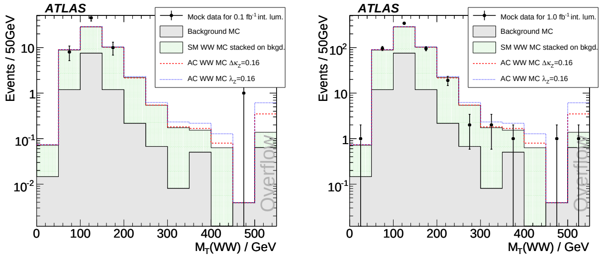
Figure 22: the MC experiment WW transverse mass distributions for 0.1 (left) and 1 \text{ fb}^{-1} (right) integrated luminosities. The last bins in the plots are 'overflow' bins.
