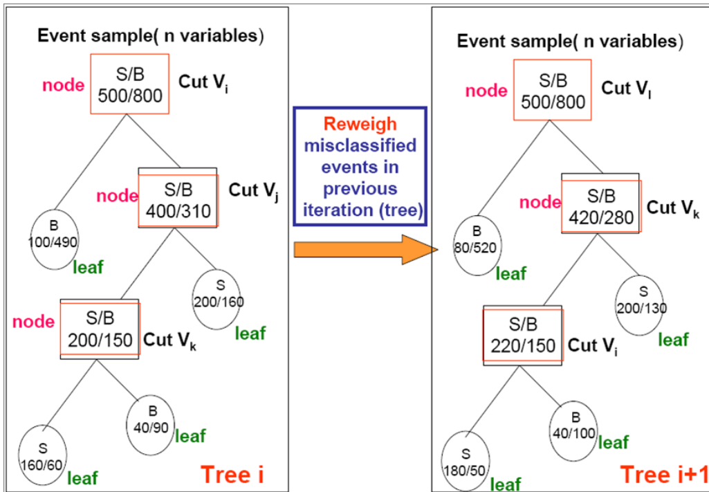
Figure 97: Diagrams for Boosted decision-trees. From Tree(i) to Tree(i+1) the mis-classified events are increased weights based on boosting algorithm. The 'note' (box) in the diagram is the variable to be split to separate signal and background in the 'decision-tree' structure. S and B denote signal and background, respectively. The 'circles' are tree leaves, depending on the signal to background ratio, those leaves are defined as signal or background leaves.
