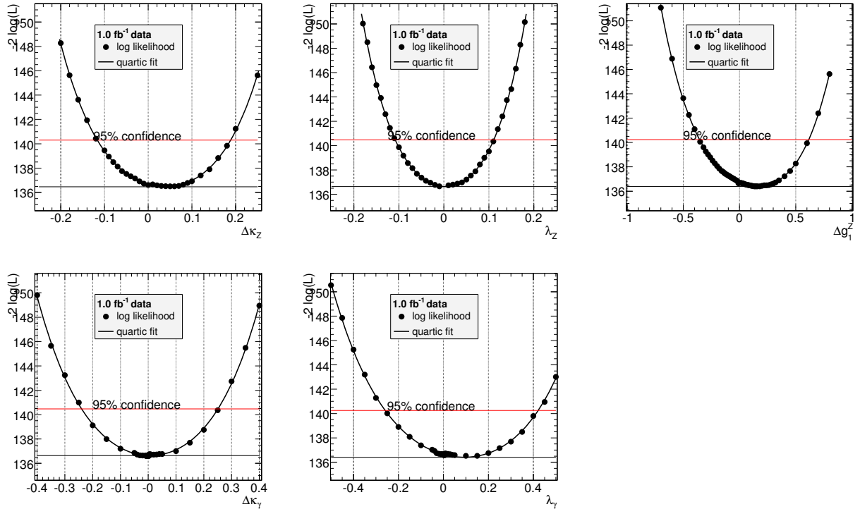
Figure 24: Anomalous coupling parameters Likelihood fitting for 1 \text{fb}^{-1} MC data.
