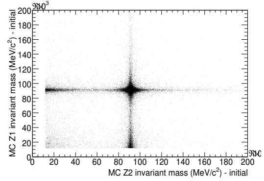
(b) Mass correlations of the two Z bosons in the PYTHIA sample. The three event types ZZ , ZZ^* and Z^*Z^* are clearly separated.
