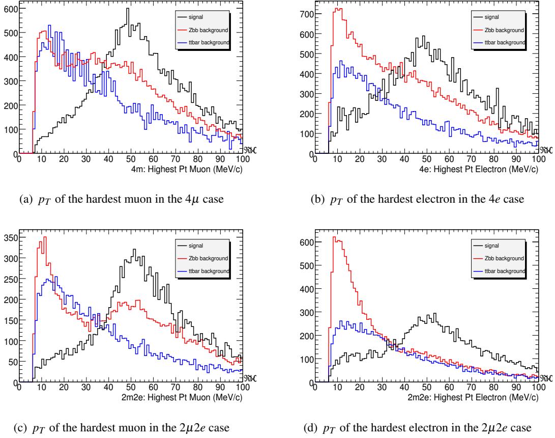
Figure 75: Max p_T discriminating variable for signal and background.
