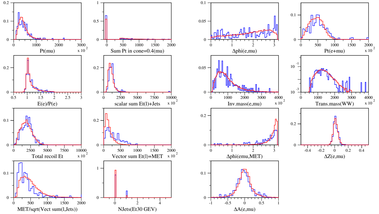
Figure 13: Distributions of the BDT training input variables after BDT selection of W^\pm W^\mp \rightarrow e^\pm \nu \mu^\mp \nu with \text{BDT} \geq 200 . The histograms are normalized to unit area, red for the W^+W^- signal and blue for the total background.
