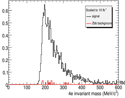
(a) Invariant mass of 4e after all cuts, for signal and Zb\bar{b} background using the tight mass cut region.
