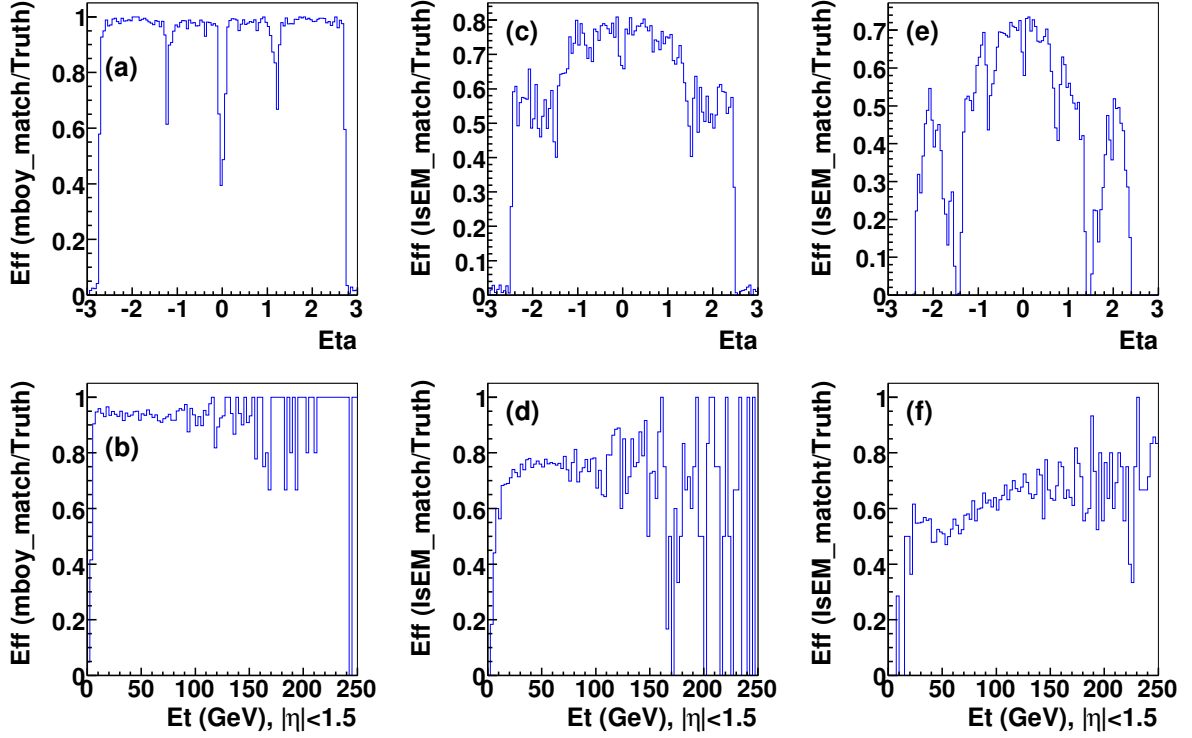
Figure 63: Reconstruction efficiencies of (a,b) muon_boy muon's, (c,d) lsEM 7x7FF electrons of Z decay, and (e,f) ISR photons of E_T(\gamma) > 25 GeV
