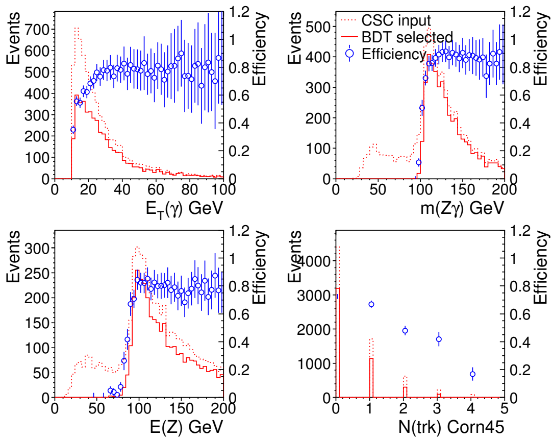
Figure 69: BDT selection efficiencies versus Z\gamma event variables for signal events with ISR photons.
