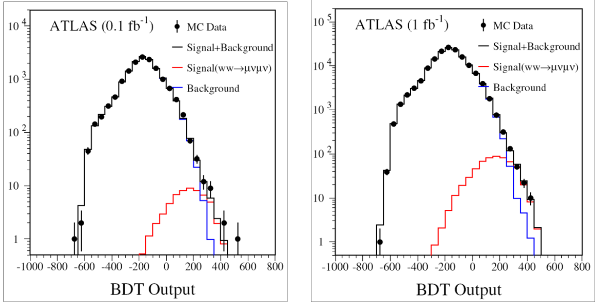
Figure 19: MC experiment BDT output spectra for W^+W^- \rightarrow \mu^+\nu\mu^-\nu detection. The left plot shows 'data' for 0.1 \text{ fb}^{-1} integrated luminosity (dots) compared to MC expected 'signal' (red histogram) and 'background' (blue histogram). The right plot shows the same for 1 \text{ fb}^{-1} integrated luminosity.
