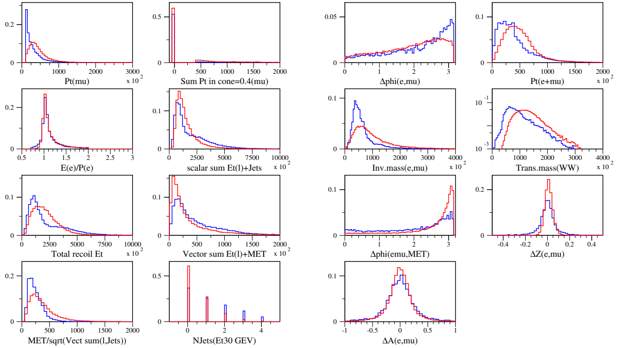
Figure 12: Distributions of the BDT training input variables for W^\pm W^\mp \rightarrow e^\pm \nu \mu^\mp \nu selection (after pre-selection). The histograms are normalized to unit area, red for the W^+W^- signal and blue for the total background.
