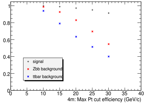
(a) Efficiency of the p_T cut
