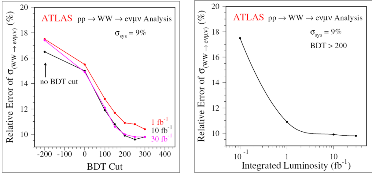
Figure 18: Left plot: the relative errors for cross section measurement as a function of the BDT cut. The optimal BDT spectrum cut should be around 200. Right plot: the relative errors as a function of integrated luminosity (with BDT spectrum cut at 200). From this plot, we see that systematic error starts to dominate after 5 \text{ fb}^{-1} integrated luminosity.
