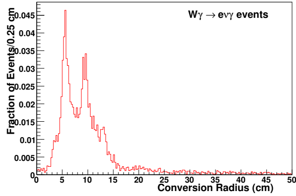
Figure 98: The radius of conversion of track pairs satisfying requirements on the two-track mass, difference in polar angle, and minimum r\phi separation.
