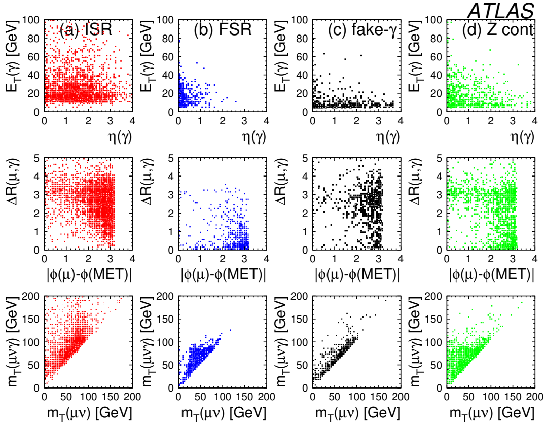
Figure 51: Distributions of W^\pm(\mu^\pm\nu)\gamma event variables, with a photon of ISR, FSR, fake background, and of inclusive Z contamination.
