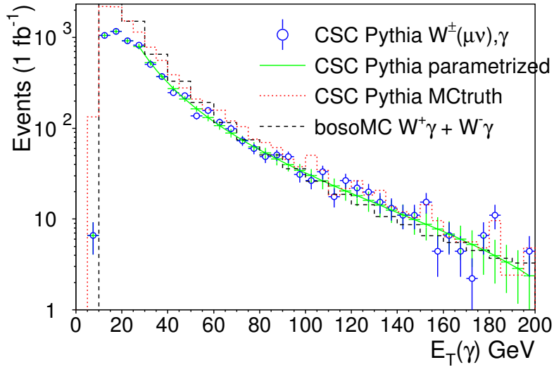
Figure 58: Distributions of E_T(\gamma) W^\pm\gamma events (points) in comparison with the Mctruth of CSC data and LO Standard Model distributions of BosoMC calculations.
