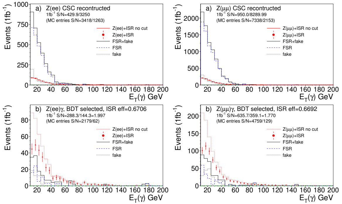
Figure 68: E_T(\gamma) distributions of reconstructed Z\gamma events (upper row) and after decision tree cuts (lower row), for Z decays into electron (left) and muon pairs (right). The distributions are normalized (by about a factor three) to the 1\text{fb}^{-1} expectation.
