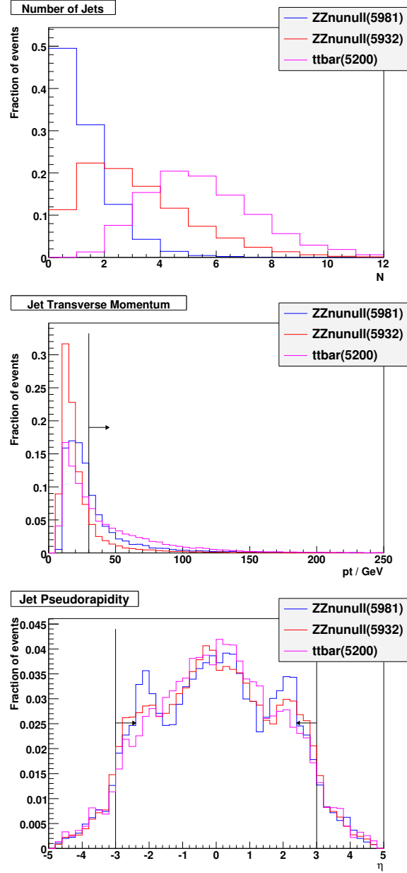
Figure 89: The jet multiplicity, p_T and \eta distributions for the version 11 signal (blue), version 12 signal (red) and t\bar{t} background. The arrows indicate the region rejected by the jet veto. The distributions are shown without cuts and normalised to unit area to compare shapes.
