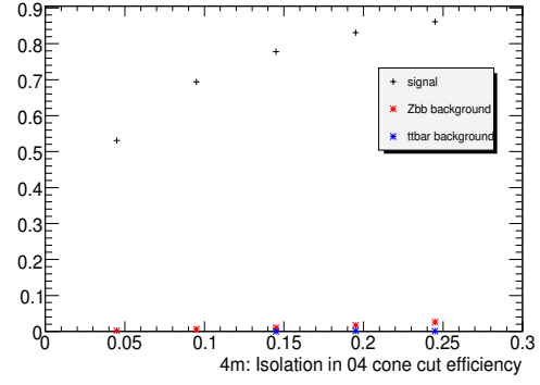
(b) Efficiency of the isolation cut
