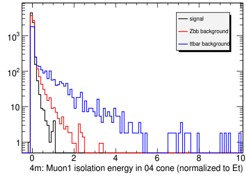
(d) Isolation variable I (see text) for the highest p_T muon
