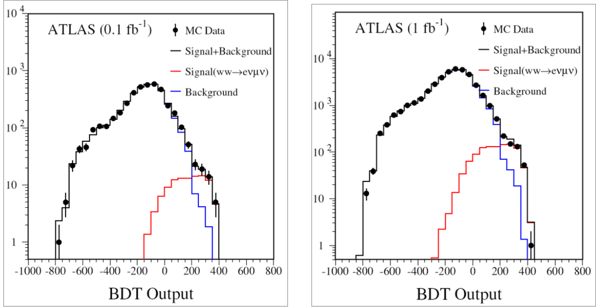
Figure 17: MC experiment BDT output spectra for W^\pm W^\mp \rightarrow e^\pm \nu \mu^\mp \nu detection. The left plot shows 'data' for 0.1 \text{ fb}^{-1} integrated luminosity (dots) compared to MC expected 'signal' (red histogram) and 'background' (blue histogram). The right plot shows the same for 1 \text{ fb}^{-1} integrated luminosity.
