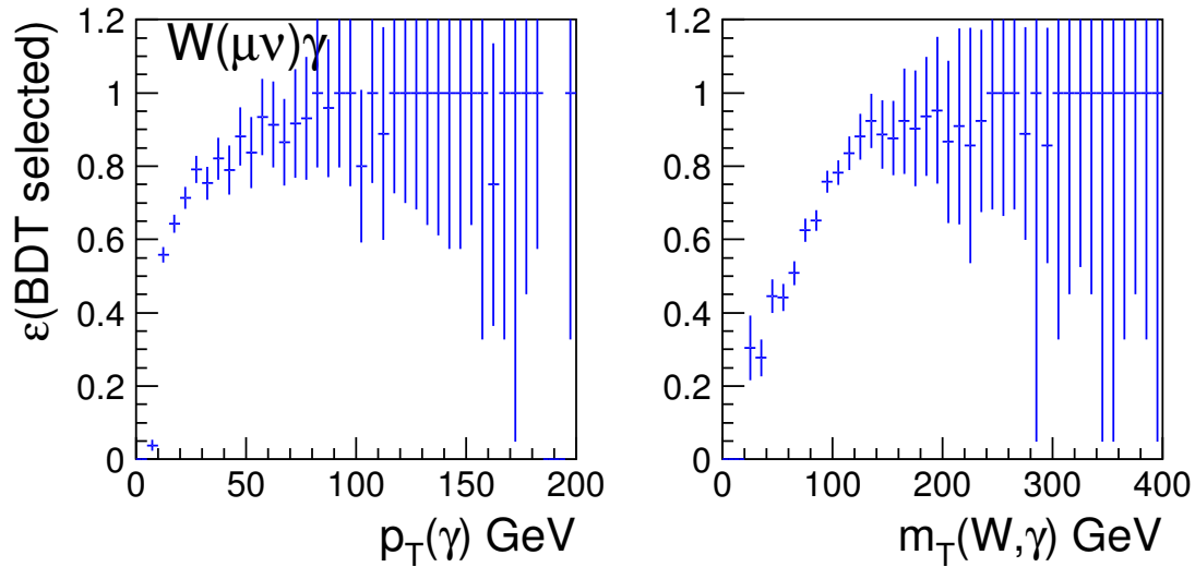
Figure 54: BDT selection efficiencies as a function of the E_T(\gamma) and the transverse mass of M_T(W^\pm, \gamma) .
