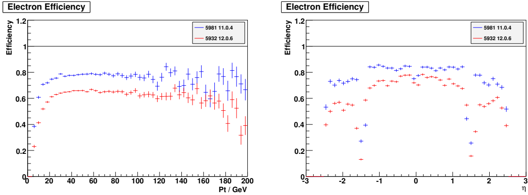
Figure 83: Electron efficiency in the signal as a function of p_T and \eta for version 11 (blue) and 12 (red) ZZ \rightarrow \ell\ell\nu\bar{\nu} signal datasets.
