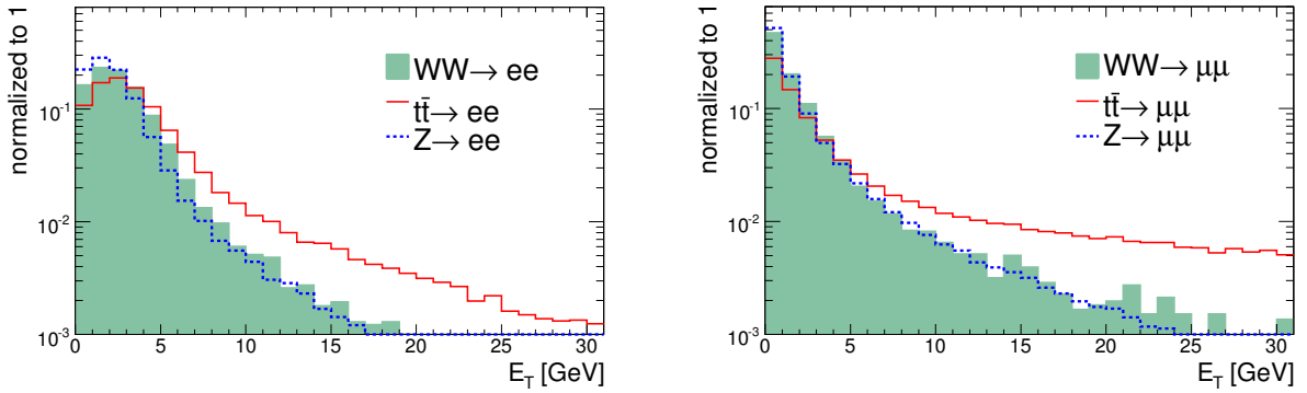
Figure 3: Transverse energy deposited in a cone \Delta R = 0.45 around the electrons ( left ) and muons ( right ).
