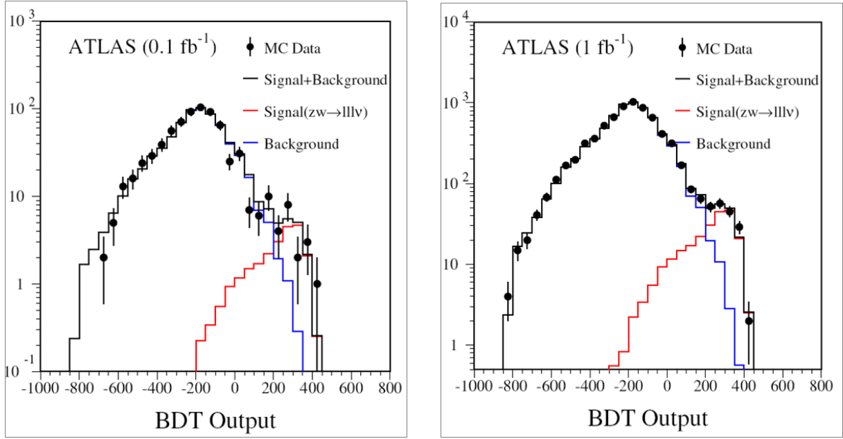
Figure 41: The Boosted-Decision-Tree output spectra for signal and background. Events are normalized to an integrated luminosity of 0.1\text{fb}^{-1} (left) and 1.0\text{fb}^{-1} (right). The points in plots are MC simulated data based on total expected mean value of signal plus background, and fluctuated with Poisson statistics.
