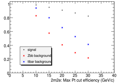
(b) Efficiency of the p_T cut for the 2\mu 2e case
