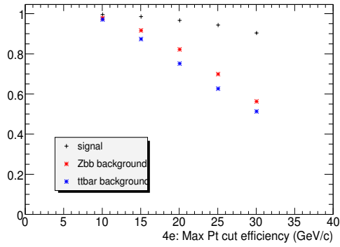
(a) Efficiency of the p_T cut for the 4e case
