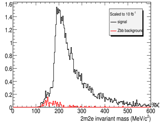
(b) Invariant mass of 2m2e after all cuts, for signal and Zb\bar{b} background using the loose mass cut region.
