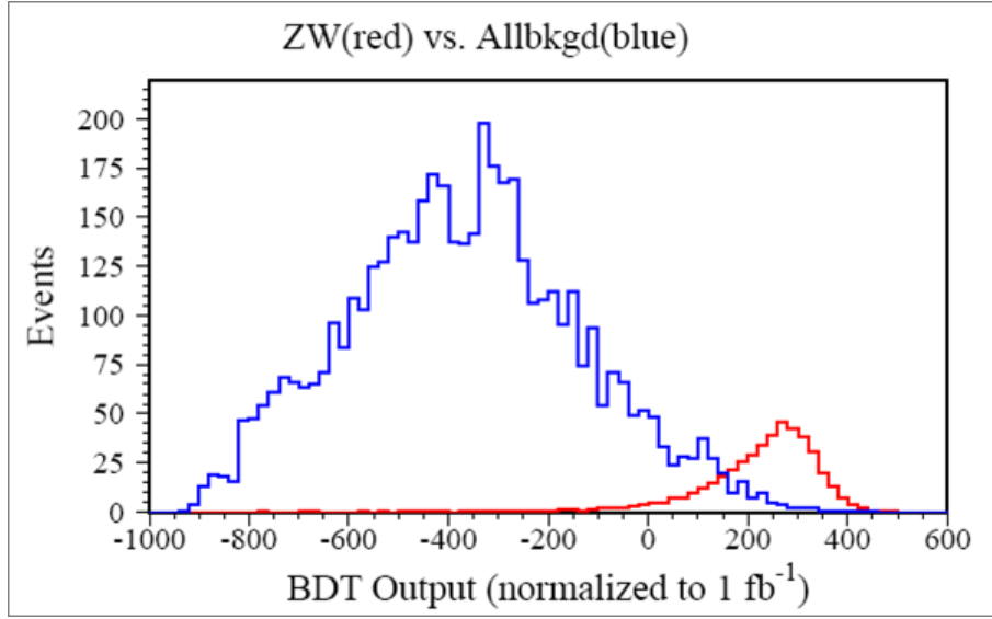
Figure 36: The BDT output distributions for signal (red histogram) and background (blue histogram). Events are normalized to an integrated luminosity of 1\text{fb}^{-1} . A cut on the BDT output > 200 , yields a signal to background ratio of about 10.
