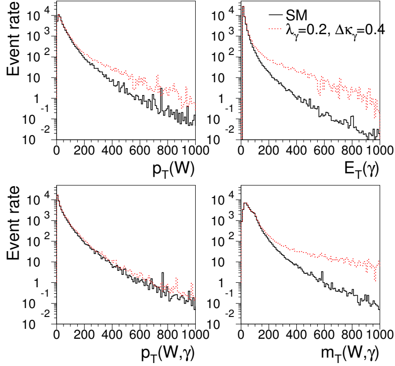
Figure 57: Distributions of transverse momenta and transverse masses of W^\pm\gamma final state particles of BosoMC calculations with \lambda_\gamma = 0.2 and \Delta\kappa_\gamma = 0.4 .
