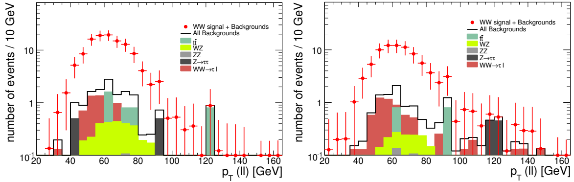
Figure 11: Transverse momentum distributions of lepton pairs after applying kinematic cuts from Selection-A (left) and Selection-B (right). The distributions are shown for sum of signal and various backgrounds, and for separated backgrounds for L=1\text{fb}^{-1} .
