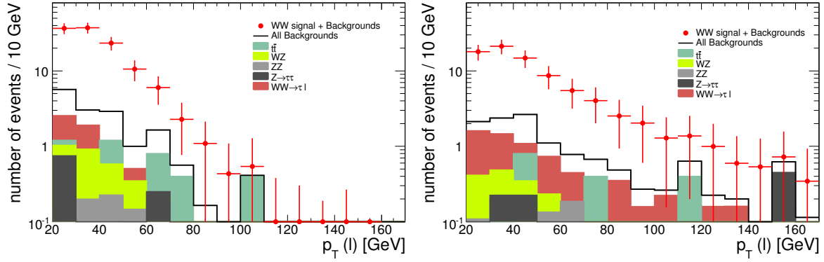
Figure 10: Transverse momentum distributions of leptons after applying kinematic cuts from Selection-A (left) and Selection-B (right). The distributions are shown for sum of signal and various backgrounds, and for separated backgrounds for L=1\text{fb}^{-1} .
