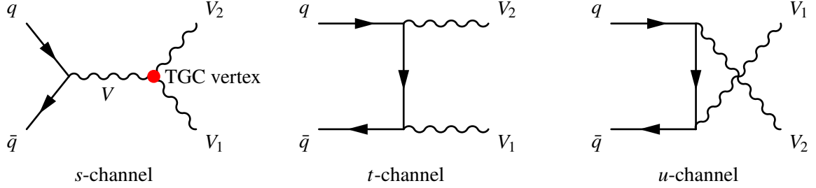
Figure 1: The generic Standard Model tree-level Feynman diagrams for diboson production at hadron colliders; V, V_1, V_2 = \{W, Z, \gamma\} . The s -channel diagram, on the left, contains the trilinear gauge boson vertex. In the Standard Model, only WW\gamma and WWZ vertices are allowed.
