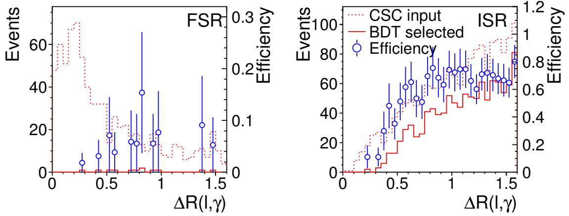
Figure 65: The opening angles in \Delta R(l^\pm, \gamma) of FSR and ISR photons to the nearest leptons (of Z(\mu^+\mu^-)\gamma events), and the selection efficiencies with Boosted Decision Tree method.
