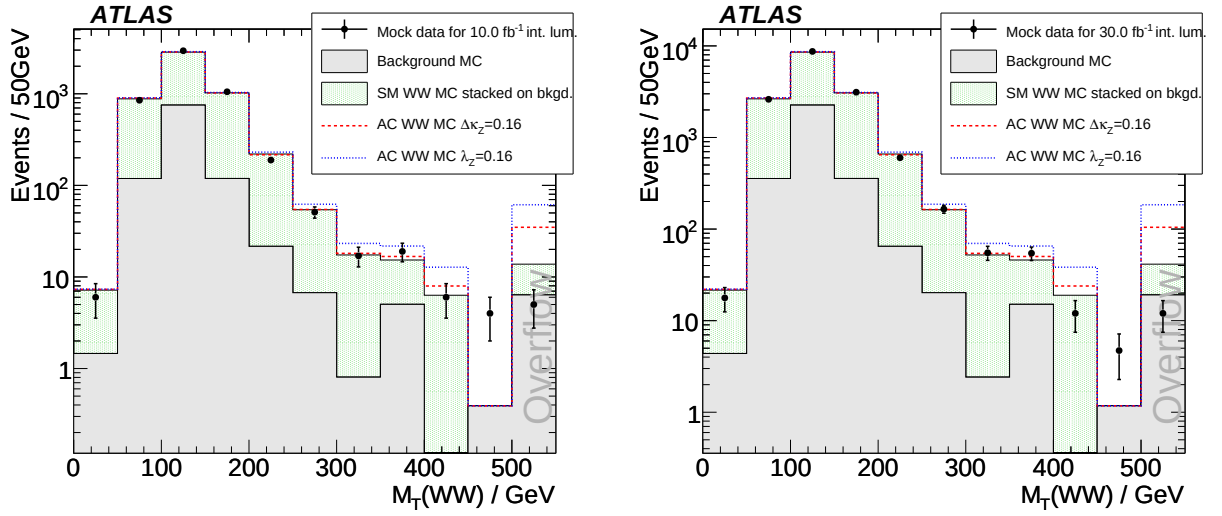
Figure 23: The MC experiment WW transverse mass distributions for 10 (left) and 30 \text{fb}^{-1} (right) integrated luminosities. The last bins in the plots are 'overflow'-bins.
