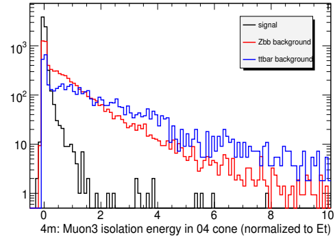
(b) Isolation variable I (see text) for the 3rd highest p_T muon
