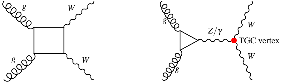
Figure 2: The Standard Model Feynman diagrams for W^+W^- production through gluon-gluon fusion in hadron colliders. Please note that the Z-exchange triangle diagrams cancel when summed over 'massless' up- and down-type contributions.
