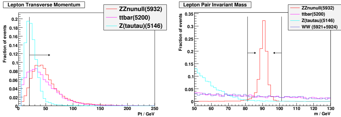
Figure 87: The lepton p_T distribution (left) and lepton pair invariant mass before cuts for the signal (red), with t\bar{t} (magenta), Z \rightarrow \tau^+\tau^- (cyan) and W^+W^- (purple) background using version 12 data. The plots are normalised to unit area for comparison of distribution shapes.
