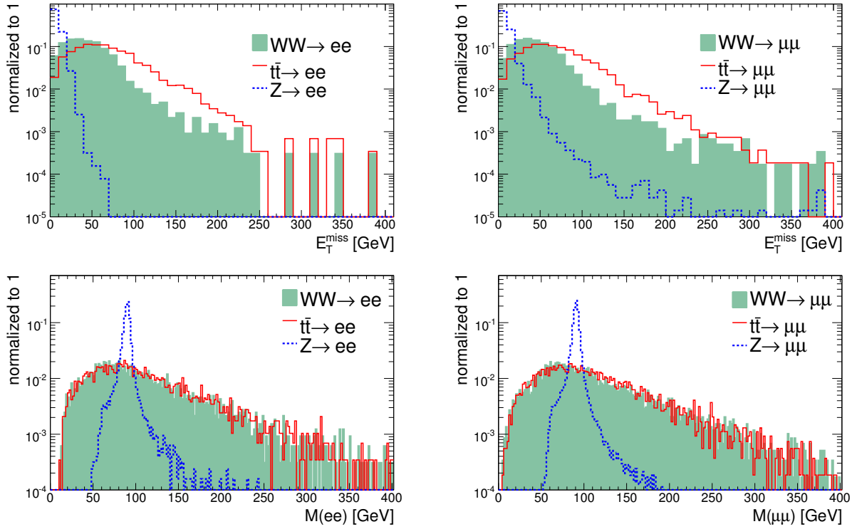
Figure 8: E_T^{\text{miss}} , and lepton invariant mass distributions for W^+W^- , t\bar{t} and Z/\gamma (Triggered events with lepton cut).
