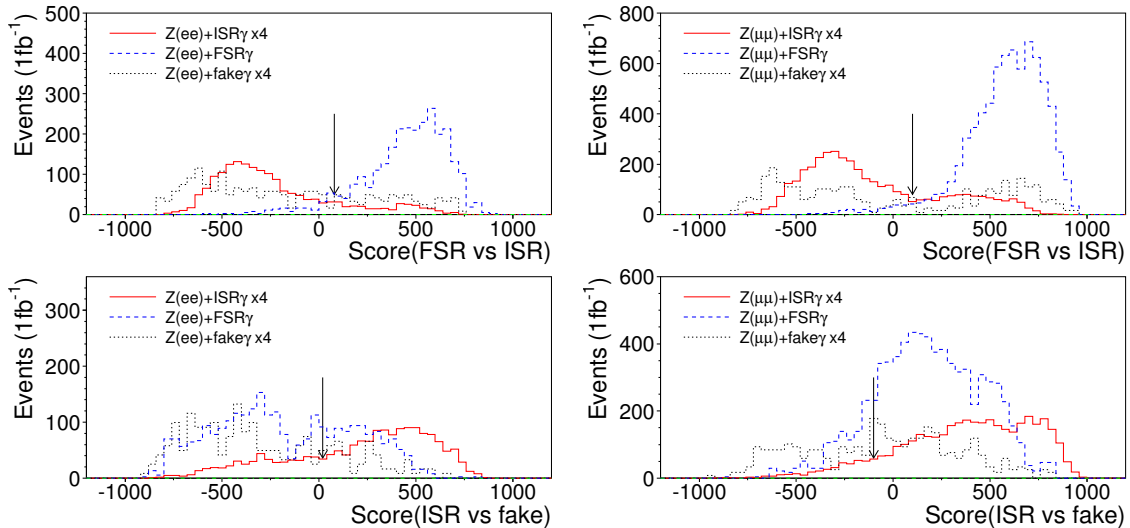
Figure 67: Test scores for the two trainings optimized for 1) FSR photons against the rest, and 2) ISR against fake photons. The arrows indicate the cuts chosen. The two columns show tests of Z to e^+e^- (left) and \mu^+\mu^- (right) separately.
