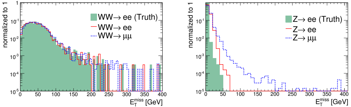
Figure 6: Comparison of truth and reconstructed \cancel{E}_T in the ee and \mu\mu channels for WW and Drell-Yan processes.
