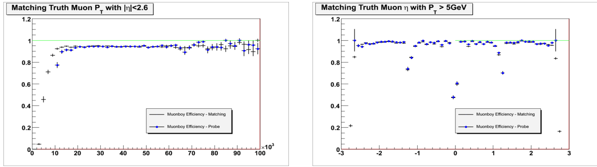
Figure 27: (a) left: the muon reconstruction efficiency as a function of muon p_T , (b) right: the muon reconstruction efficiency as a function of rapidity \eta .
