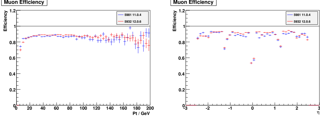
Figure 86: Muon efficiency as a function of p_T and \eta for version 11 (blue) and 12 (red) ZZ \rightarrow \ell\ell\nu\bar{\nu} signal datasets.
