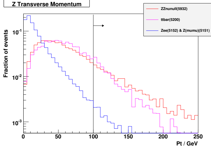
Figure 90: The p_T(Z) distribution for the version 12 signal (red), Z \rightarrow \ell^+ \ell^- (blue) and t\bar{t} (magenta). Plots are shown without applying cuts and are normalised to unit area.
