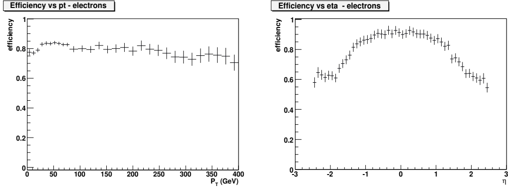
(a) p_T dependence of the electron reconstruction efficiency in ZZ events (b) \eta dependence of the electron reconstruction efficiency in ZZ events
