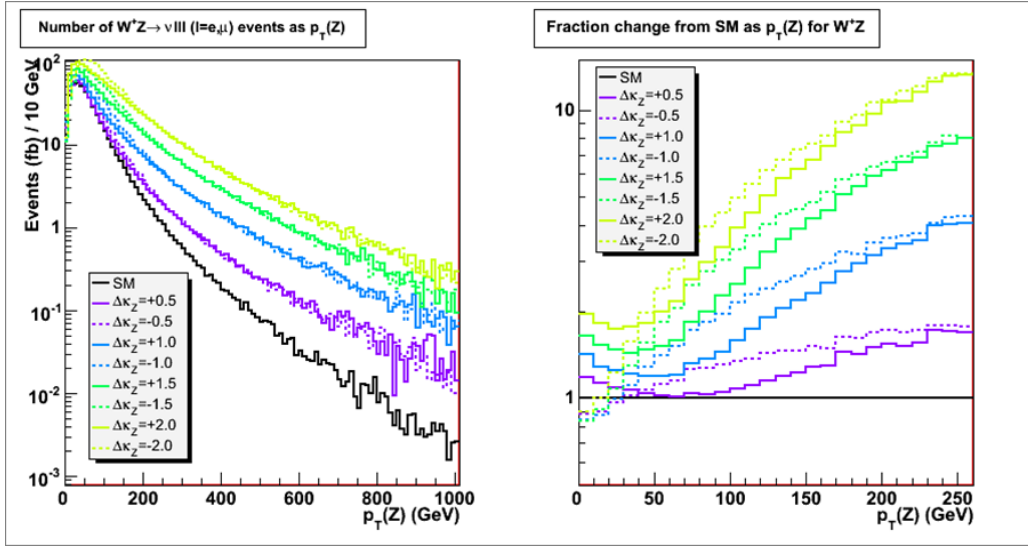
Figure 43: Left plot, The p_T(Z) distributions for different WWZ couplings ( \Delta\kappa_Z ) and right plot, the differential cross section ratio, d\sigma(\text{non-SM})/d\sigma(\text{SM}) .
